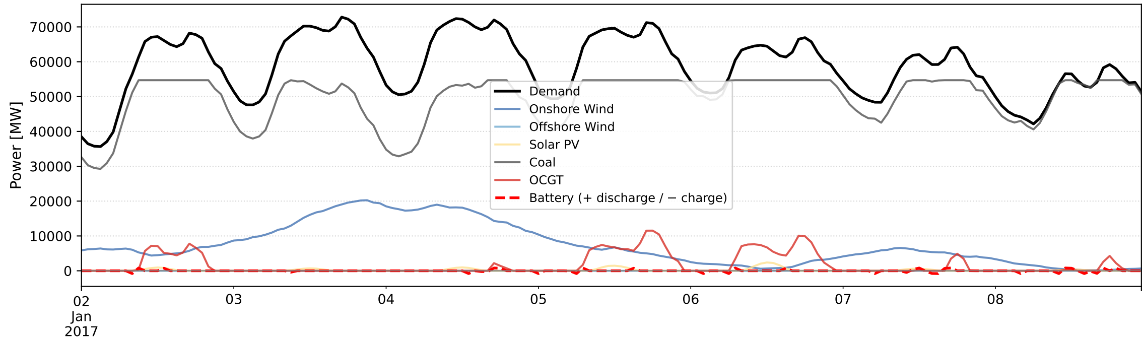
Germany 2017 — Demand, Generation and Battery (Winter week Jan 2-8)
